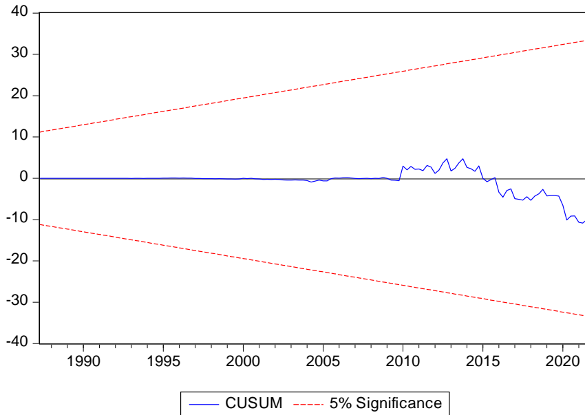
Fig 1: CUSUM Stability test of ARDL (5,5,1,0,2,0) model
