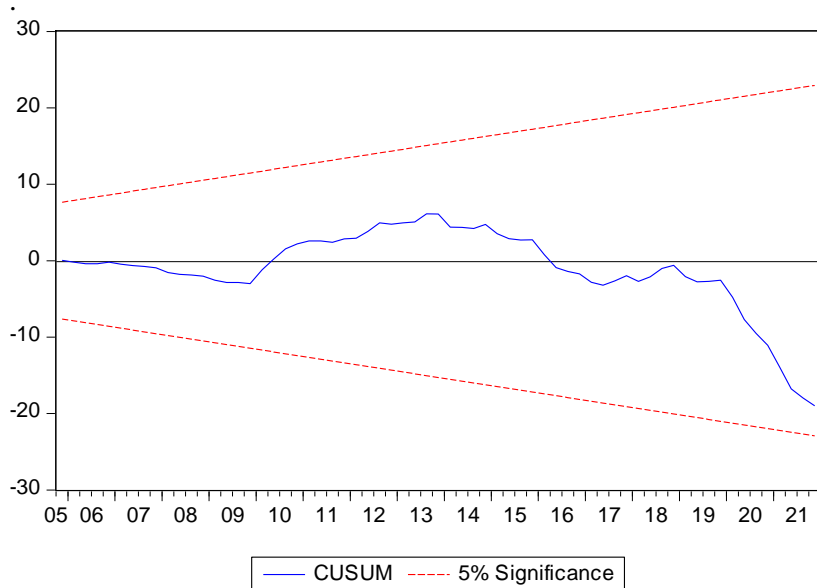
Fig 2: CUSUM Stability test of ARDL (5,5,1,0,2,0,0) model
